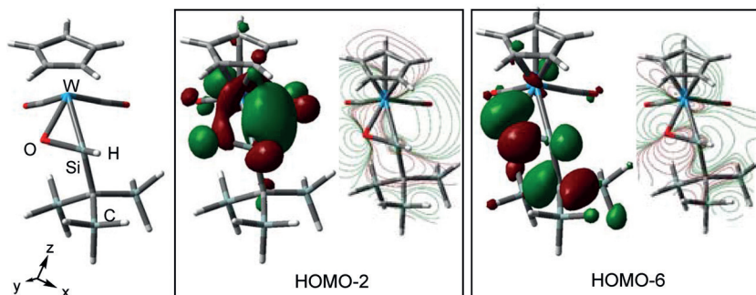
Figure 4. Optimized structure (left) and important Kohn–Sham orbitals of 2' (middle and right).
